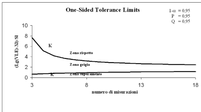
Figura B4 - Curve OTL
